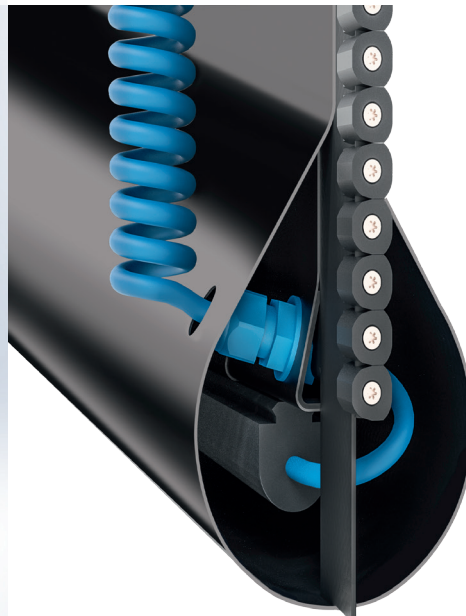
Bottom edge detection via intrinsic safety barrier
