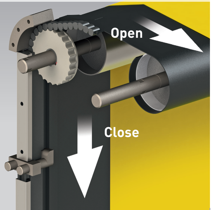
"PUSH-PULL PT " Drive Technology
